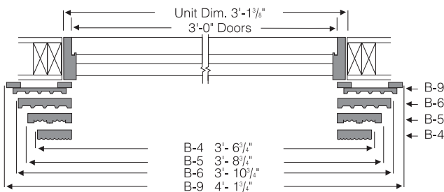
Single Door Unit
