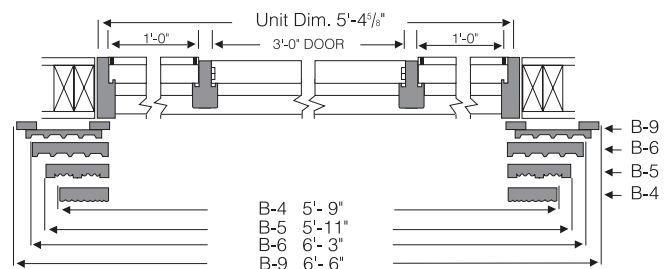
Single Door with two 1'-0" Sidelights (Mull post)
