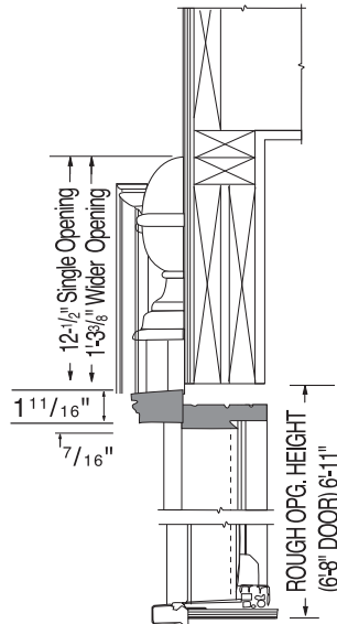
Basic Trim w/Pediment Head
