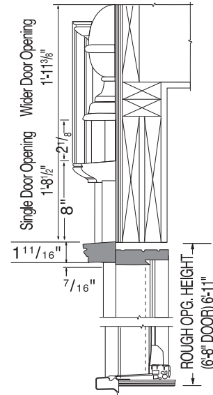
Basic Trim w/Pediment Head & Frieze Board
