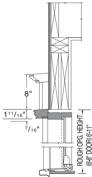
Basic Trim w/Frieze Board
